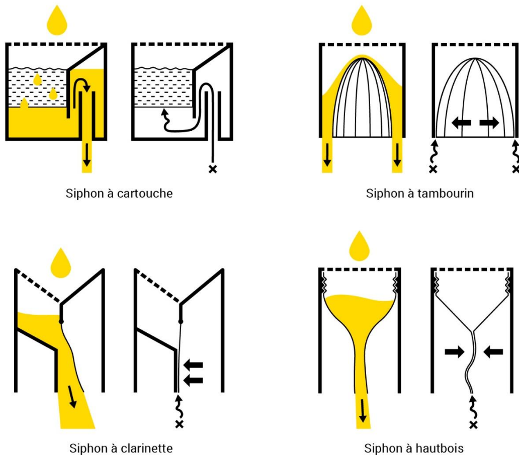
Figure 2 : Siphons secs
